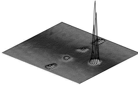
Figure 8. The density of the kinetic energy in a simulation just after the soliton has passed the hole. T = 150 , v_{in} = 1.9165 .
