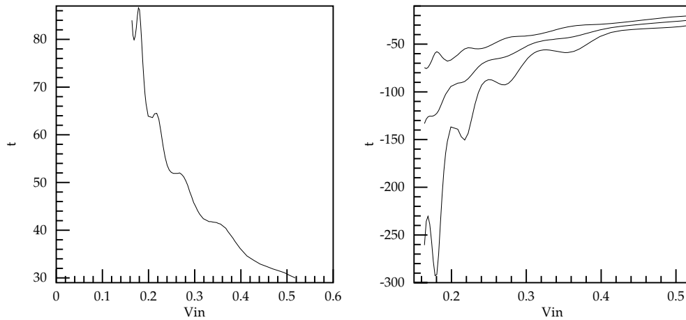
Figure 7. Left: time spent in the hole; right: time in the hole minus the time needed to traverse the hole with various velocities. Top curve: initial velocity, middle curve: average, bottom curve: outgoing one.
