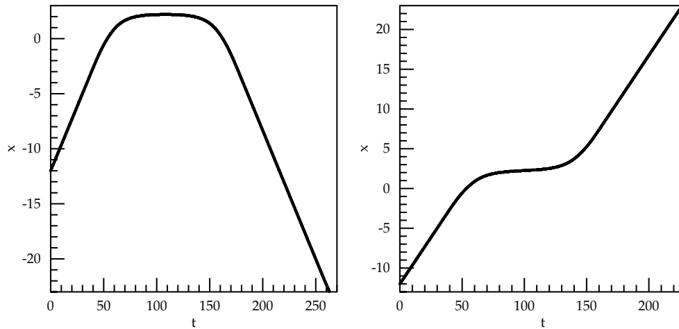
Figure 3. Time dependence of the position of the soliton initially placed at x = -12 : left v < v_{cr} , right v > v_{cr} .
