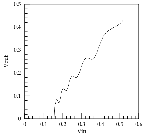
Figure 6. Velocities of transmitted solitons, x axis—incoming, y axis—outgoing
