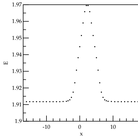
Figure 1. Energies of our basic soliton as a function of its position.
