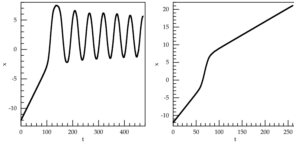
Figure 5. Time dependence of the position of the soliton initially placed at x = -12 : left, v < v_{cr} ; right, v > v_{cr} .
