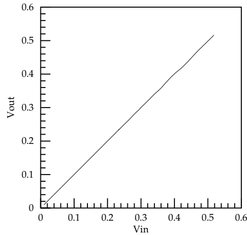
Figure 2. Soliton velocities, x axis—incoming, y axis—outgoing.
