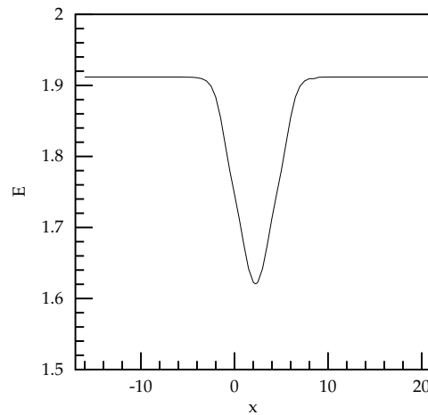
Figure 4. Energies of our basic soliton as a function of its position.
